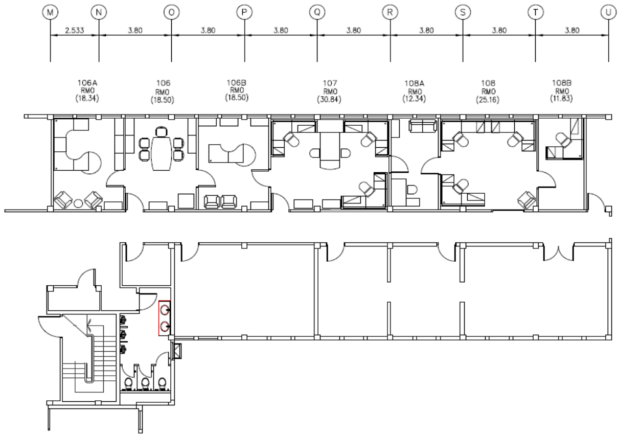
1 RMO - EXISTING FURNITURE PLAN SCALE NTS
